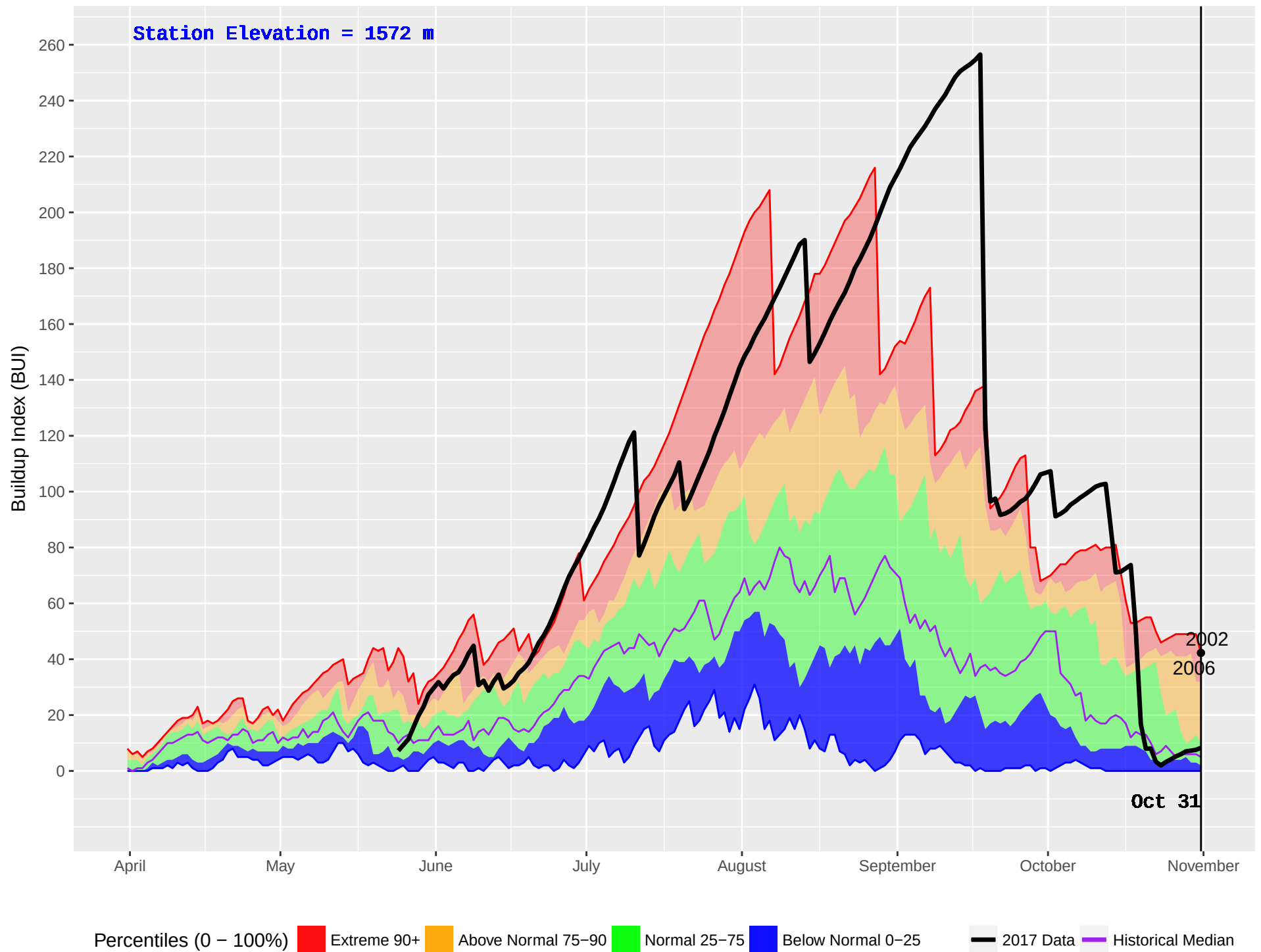
NEGRO CREEK (789) : Historical (2001–2016) and Current (2017) Noon Buildup Index (BUI)
