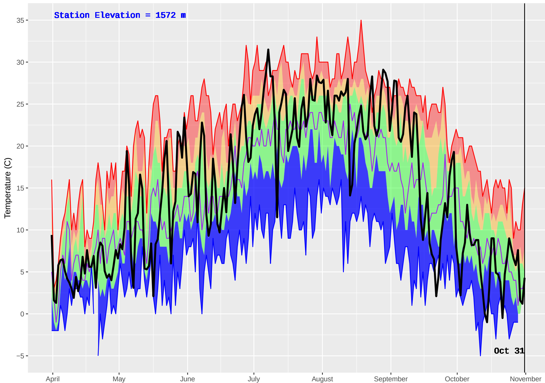
NEGRO CREEK (789) : Historical (2001–2016) and Current (2017) Noon Temperature
