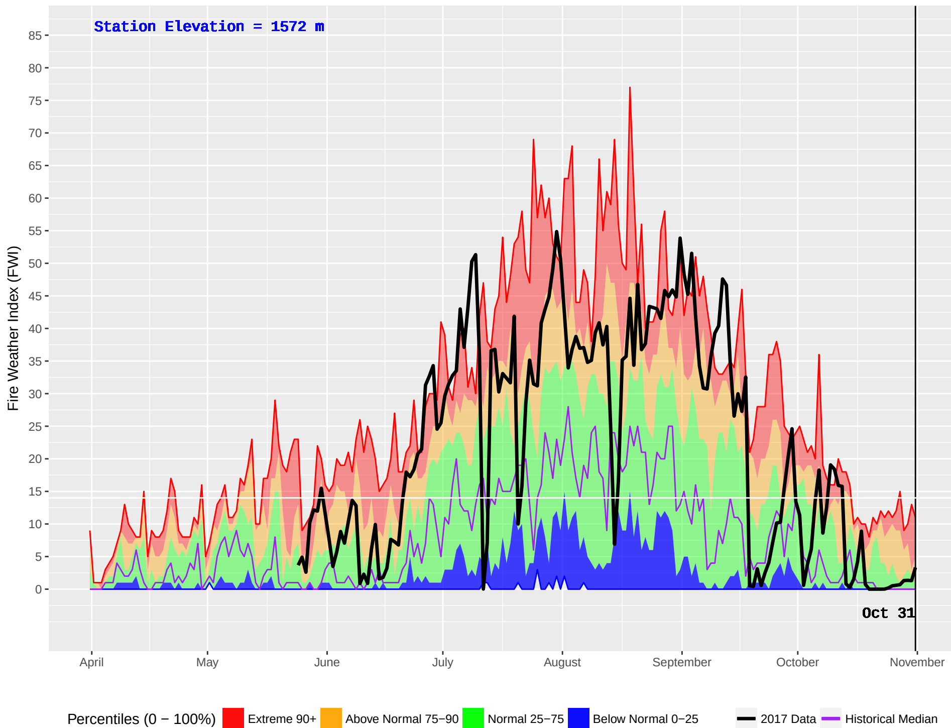
NEGRO CREEK (789) : Historical (2001–2016) and Current (2017) Noon Fire Weather Index (FWI)
